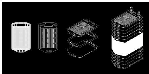
Cell Stack
