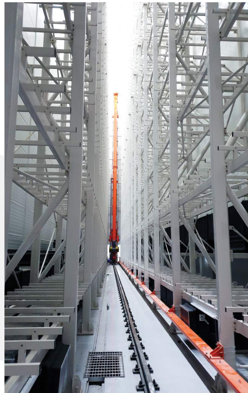
Pallet/Bucket Type System
